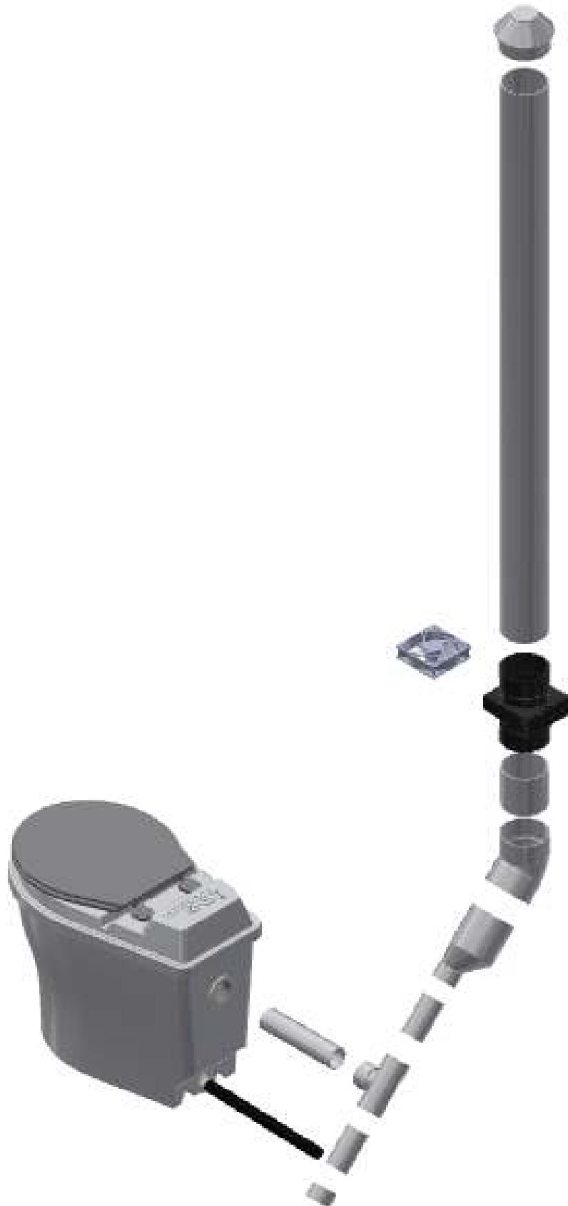
Figure 3: Ventilation pipe components break-out view
